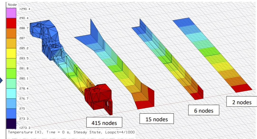
Thermal Model
